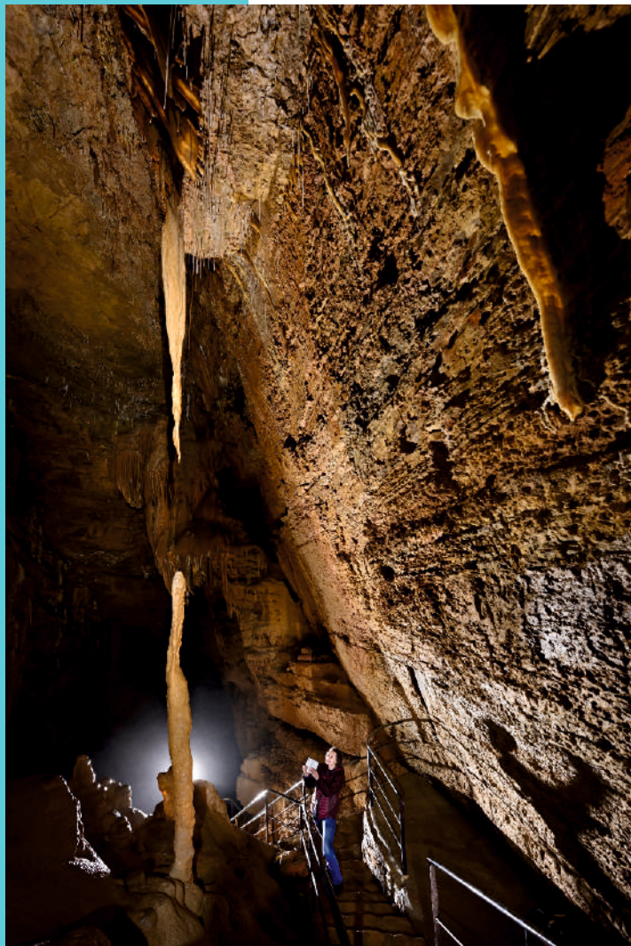
Stalactites, stalagmites
